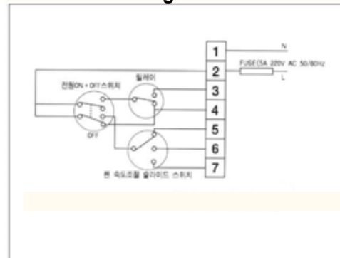
Fig 3. Internal wiring
