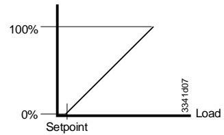
Direct acting sequence (application No.: 70...79)
